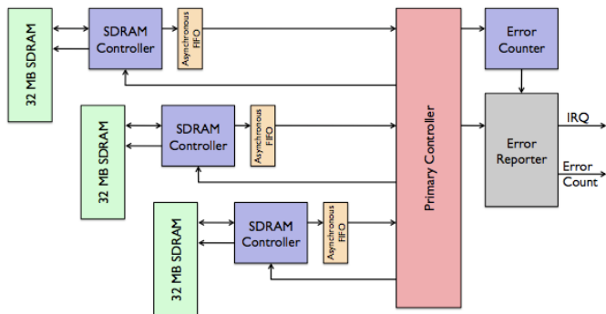
Fig. 11. SDRAM scrubber
