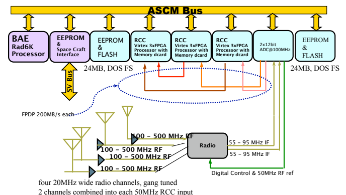
Fig. 1. Payload Block Diagram
